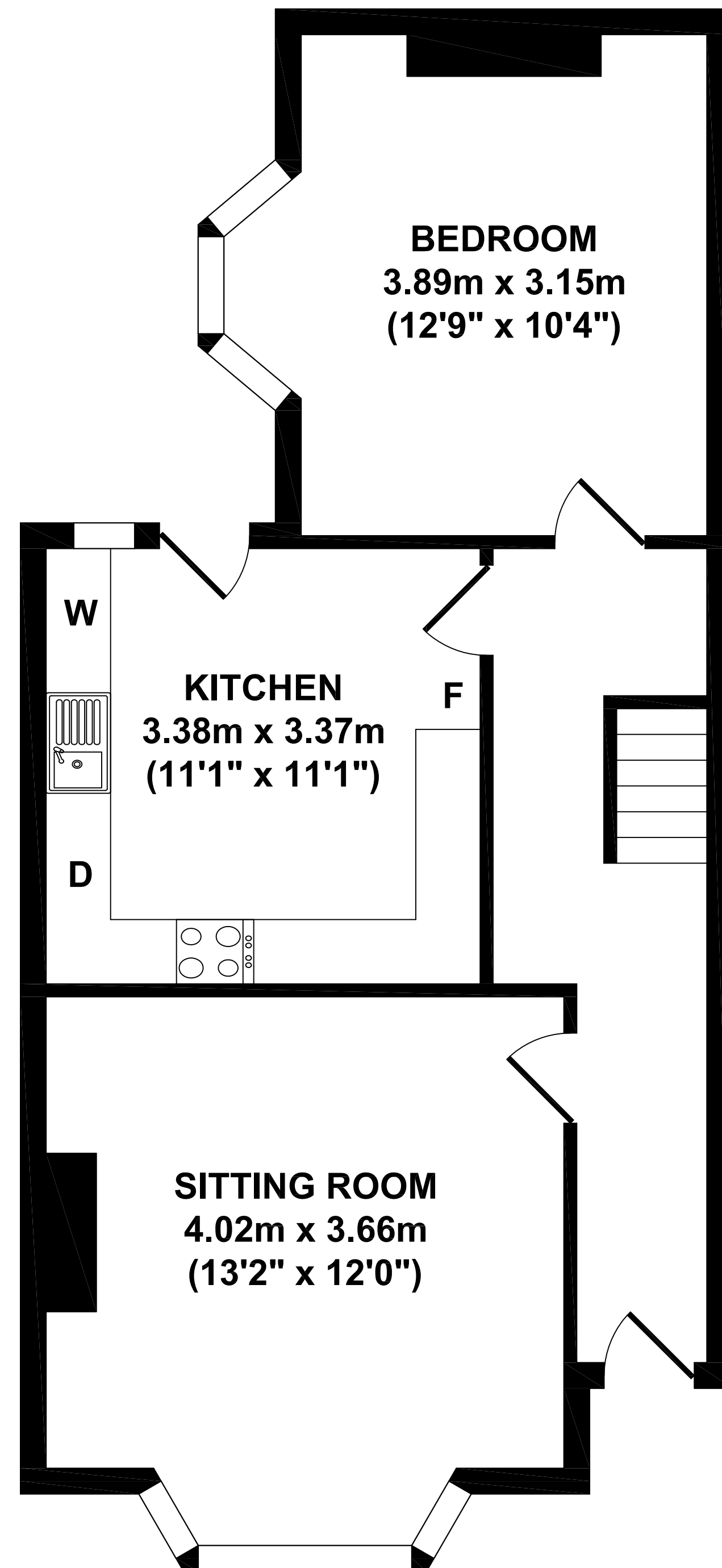
GROUND FLOOR
